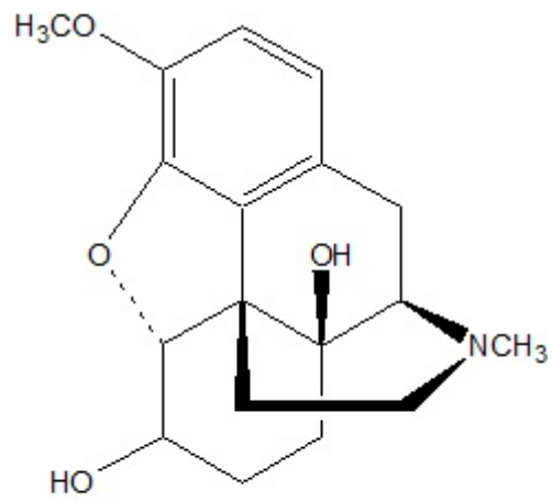
14-Hydroxydihydrocodeine
